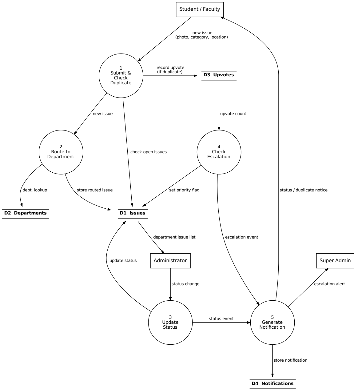
Figure 2.5: Level-1 data flow diagram decomposing the system’s major processes.
