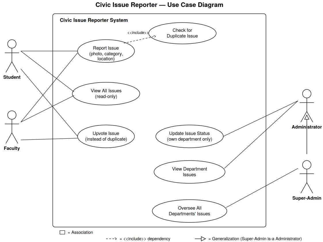
Figure 2.2: Use case diagram for the Civic Issue Reporter system.
