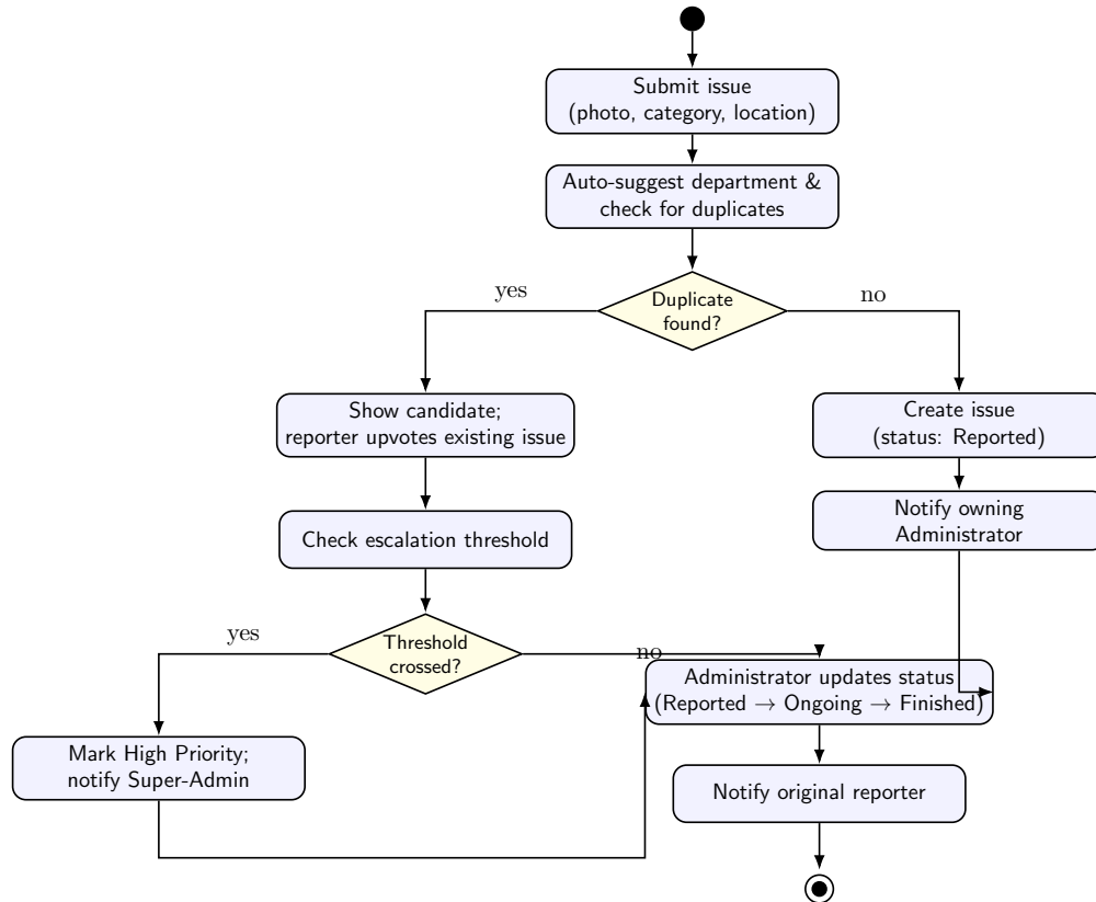
Figure 2.6: UML activity diagram for the core issue reporting and resolution workflow.
