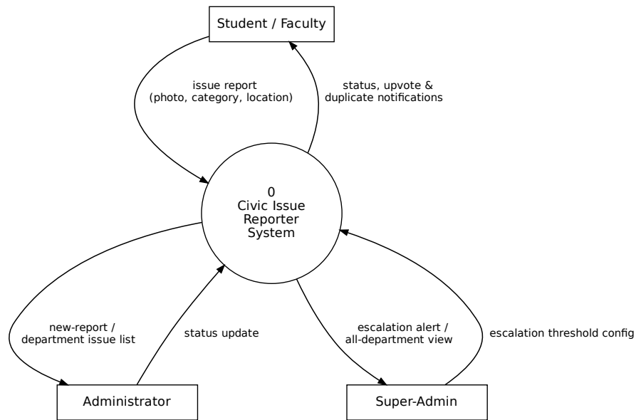
Figure 2.4: Context (Level 0) data flow diagram.
